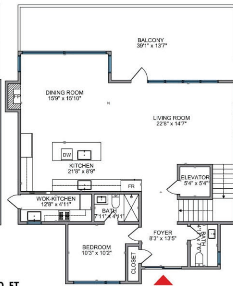
Main Floor - 1396 SQ. FT Ceiling height - 9'6"
