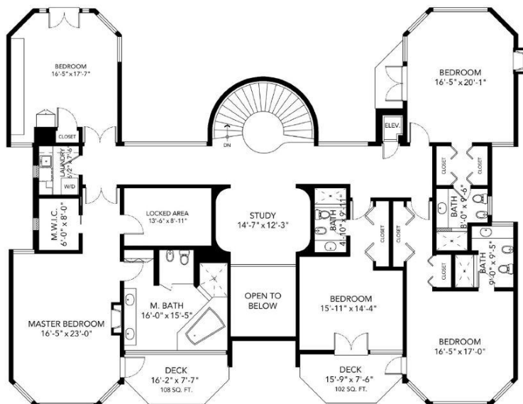
UPPER FLOOR PLAN 3527 SQ. FT.*
