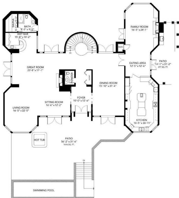
MAIN FLOOR PLAN 3564 SQ. FT.
