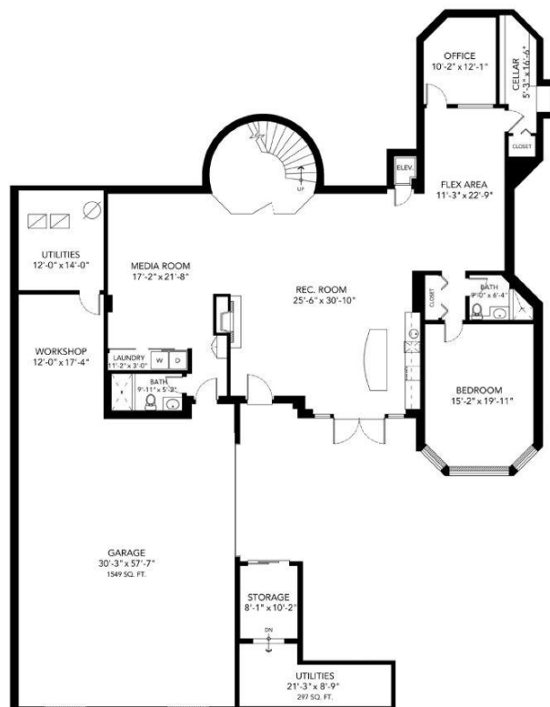
LOWER FLOOR PLAN 2811 SQ. FT. Ceiling Height: 8'-8"
