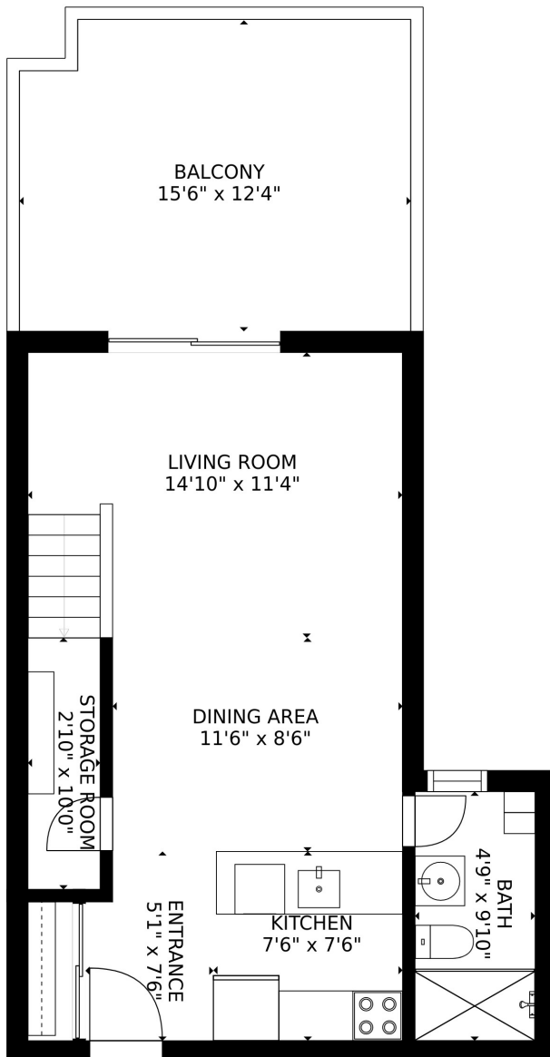
MAIN FLOOR
