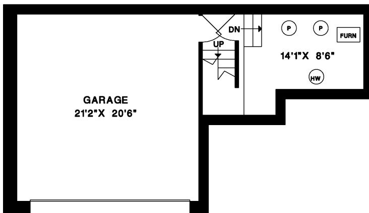
BASEMENT
