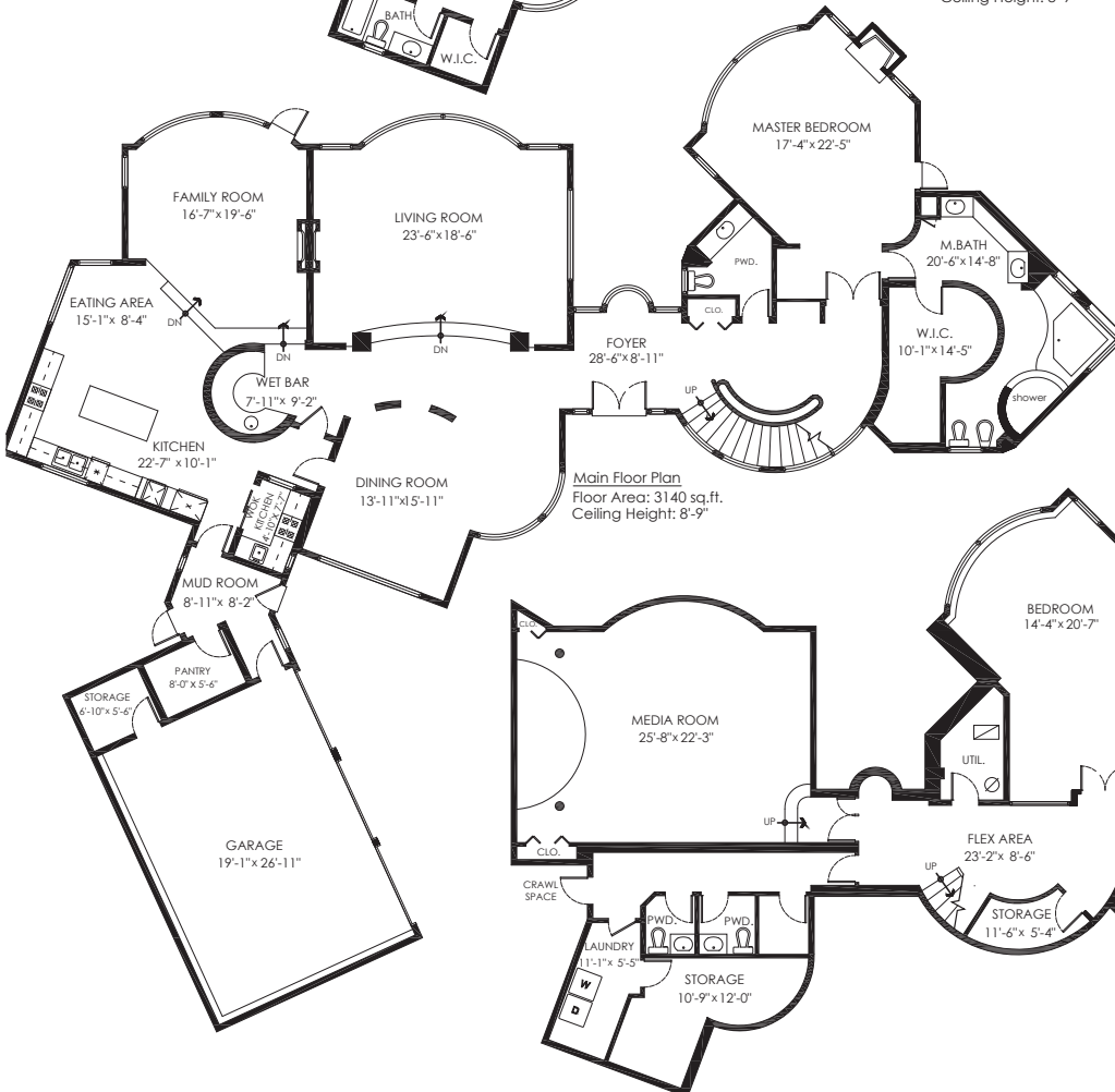
Upper Floor Plan Floor Area: 1996 sq.ft. Ceiling Height: 8'-9"
