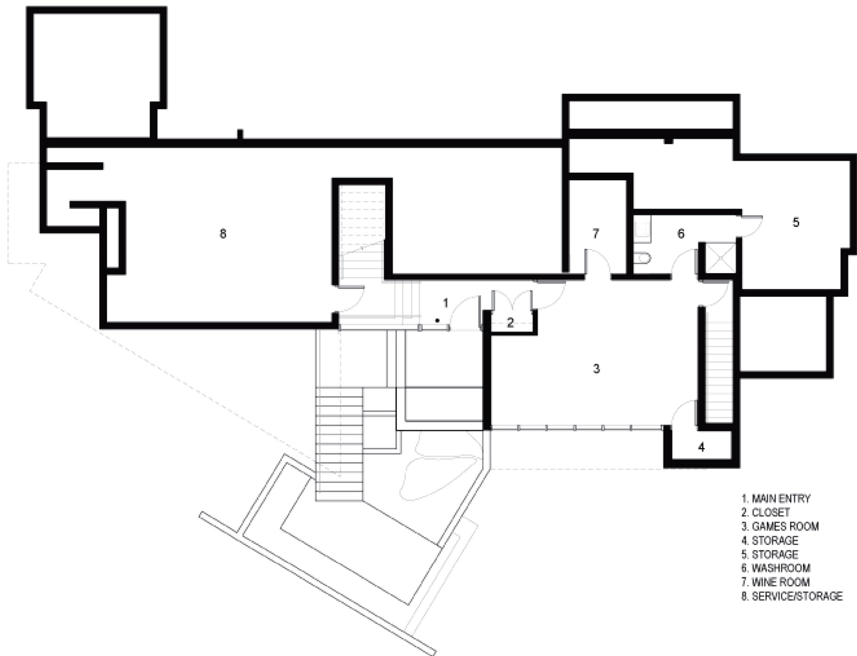
BASEMENT PLAN
