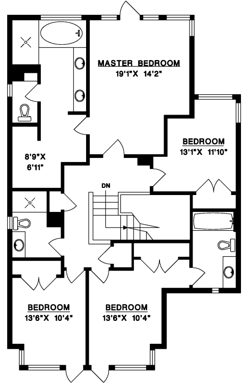
UPPER FLOOR
