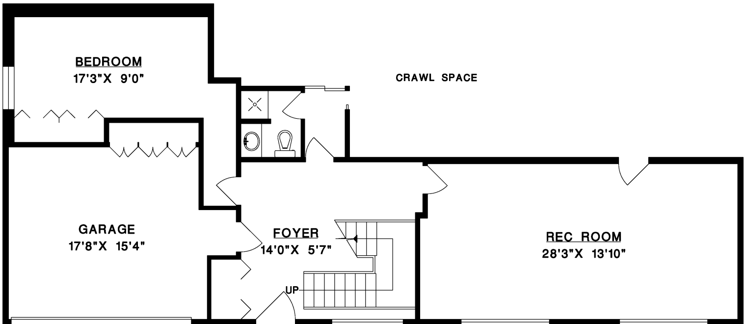
LOWER FLOOR
