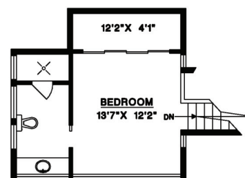
UPPER FLOOR
