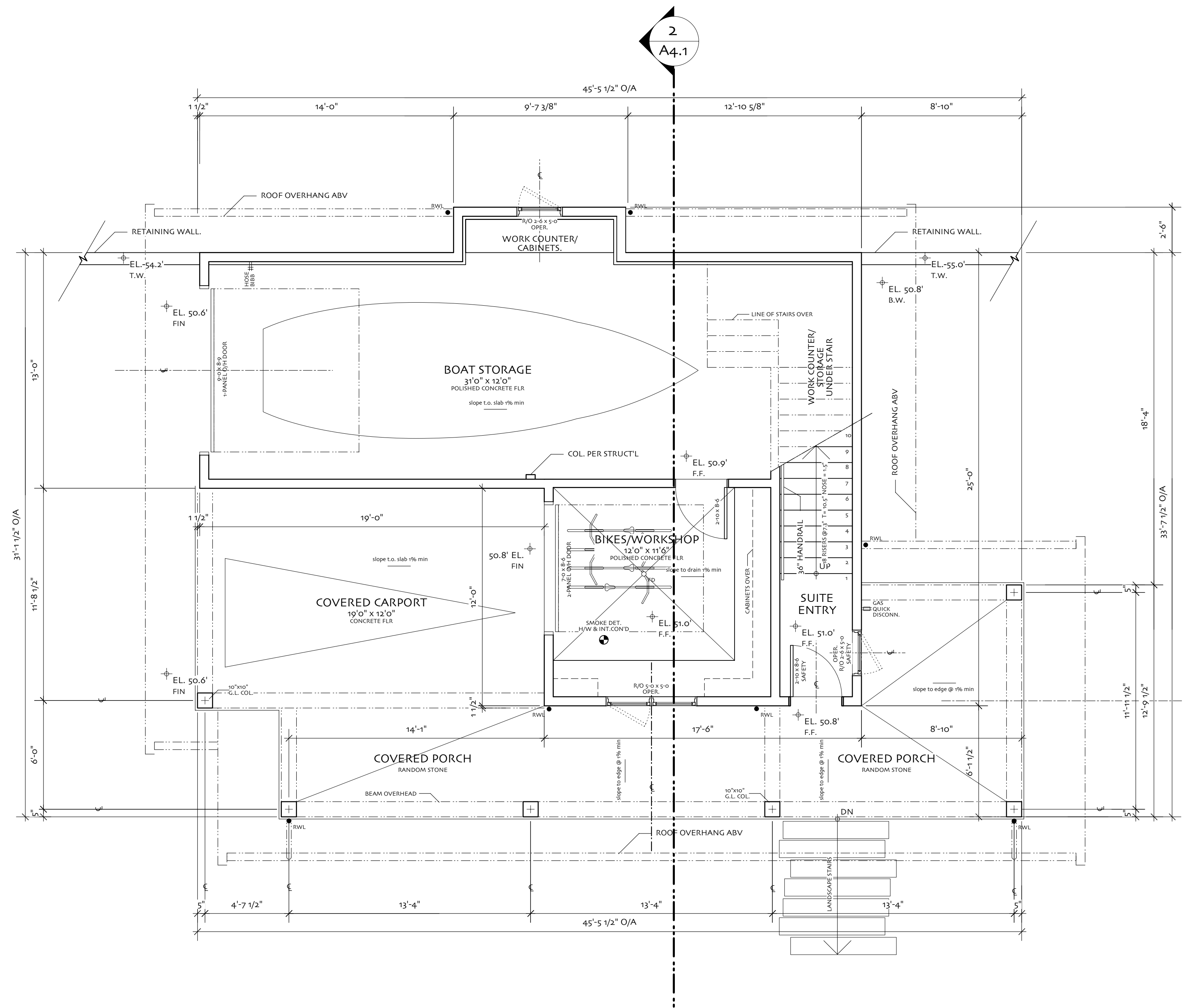
COACH HOUSE MAIN FLOOR
