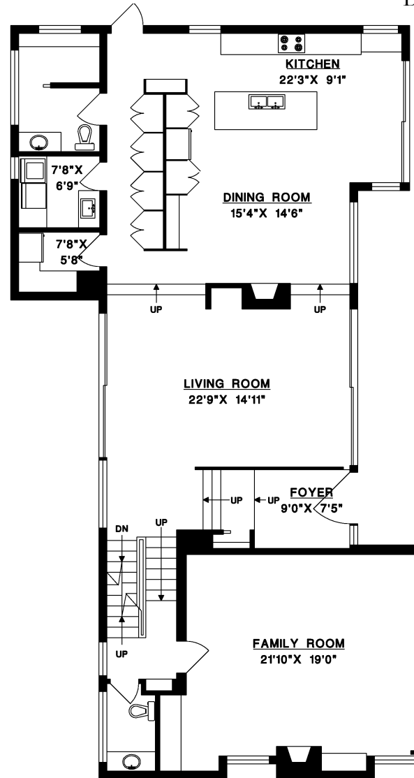
MAIN FLOOR
