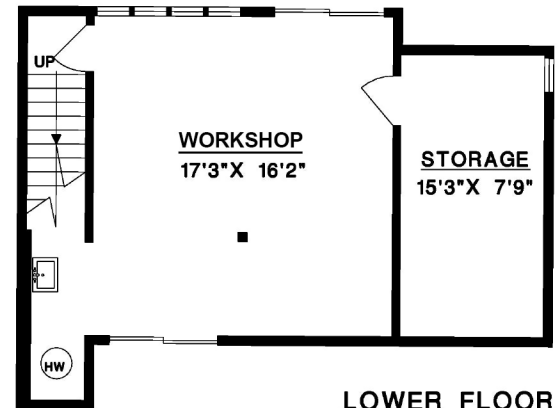
LOWER FLOOR
