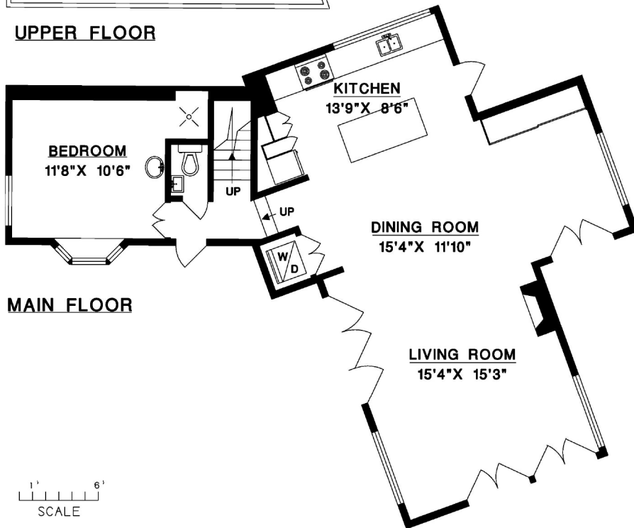
MAIN FLOOR
