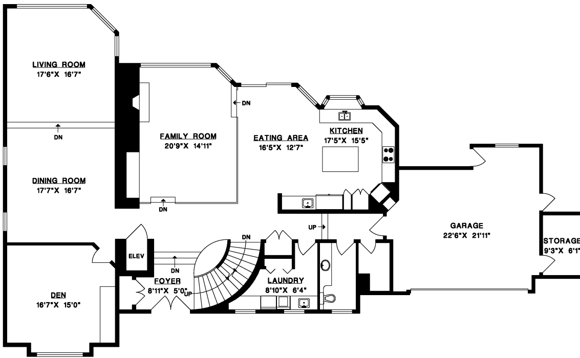
MAIN FLOOR
