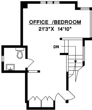
UPPER FLOOR
