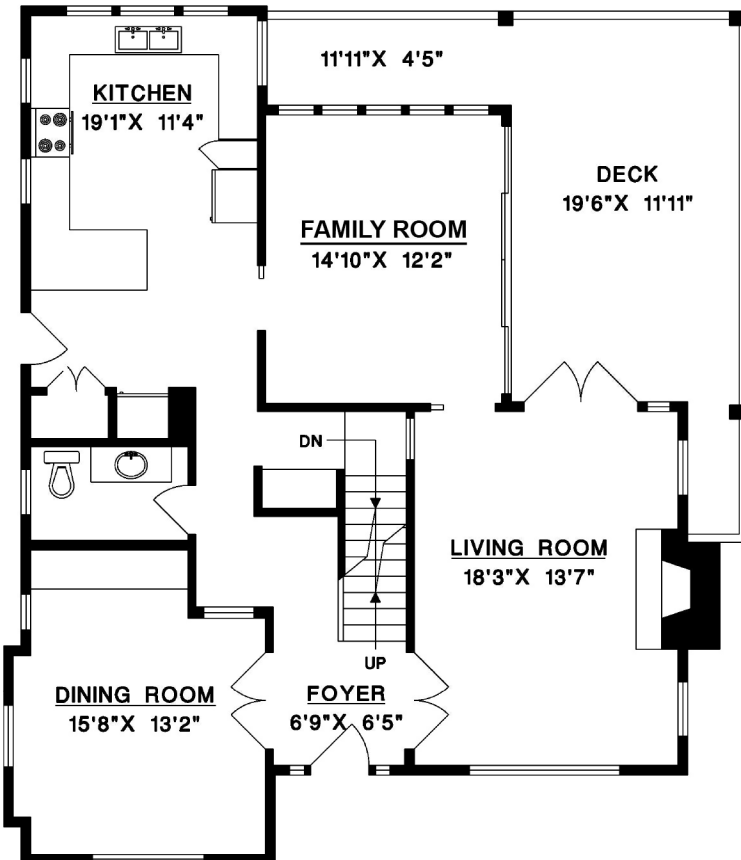
MAIN FLOOR
