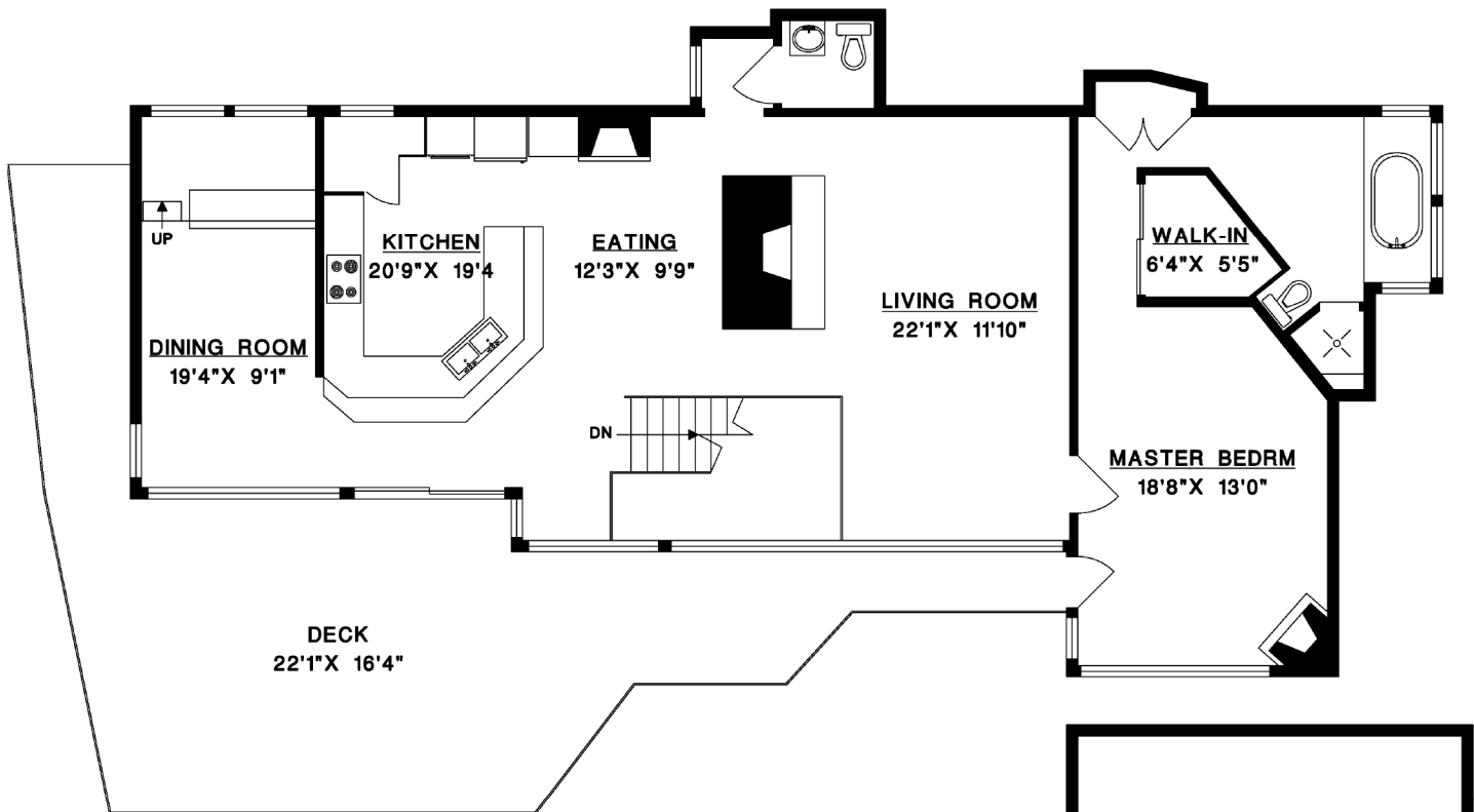
MAIN FLOOR
