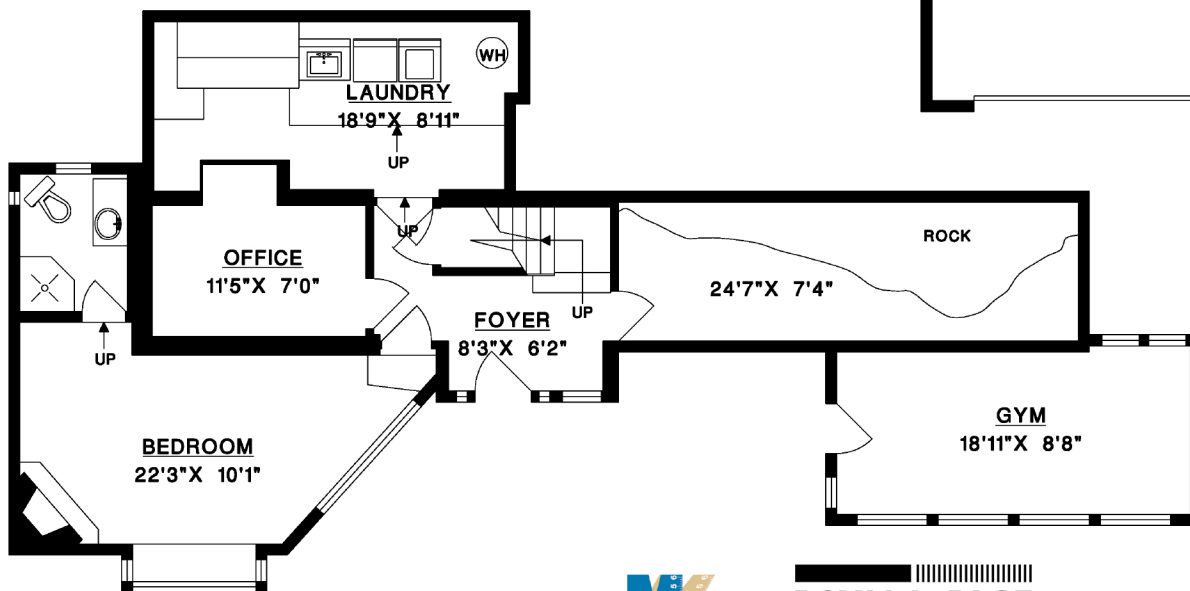
LOWER FLOOR
