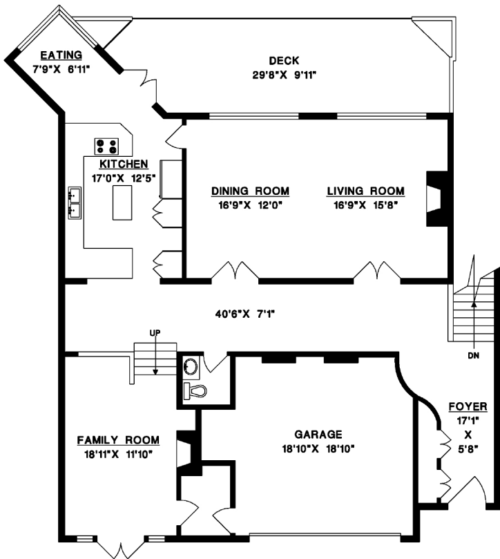
MAIN FLOOR
