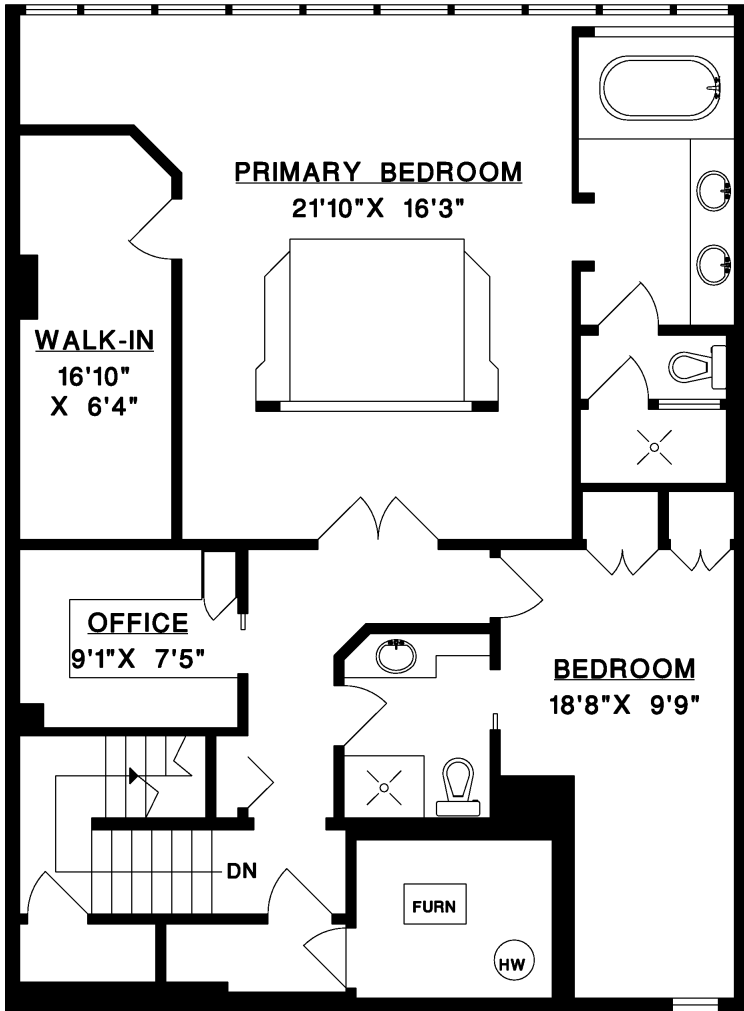
UPPER FLOOR
