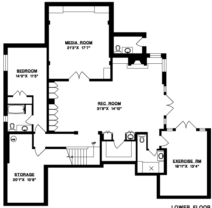
LOWER FLOOR
